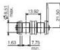
ATTACHMENT TYPE 1010
